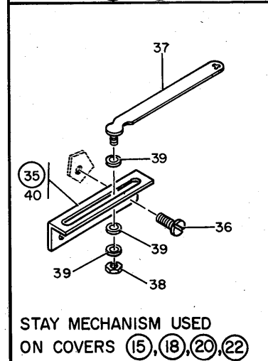
FIGURE 1. 7201-02 COVERS AND PANELS (SHEET 1 OF 3. INDEX NOS. 1-57)
