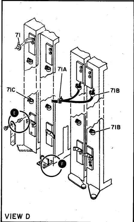
FIGURE 12. CPU FINAL ASSEMBLY-FRAME 02. (SHEET 1 OF 2, INDEX NOS. 1-97)
