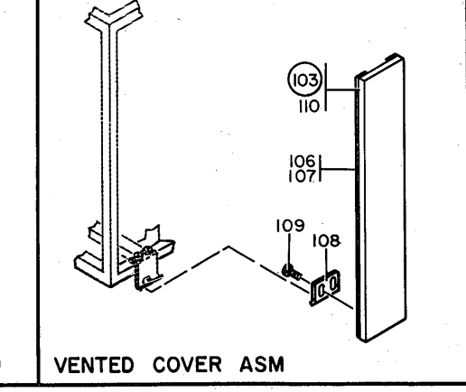
FIGURE 1. 7201-02 COVERS AND PANELS (SHEET 2 OF 3. INDEX NOS. 58-113)
