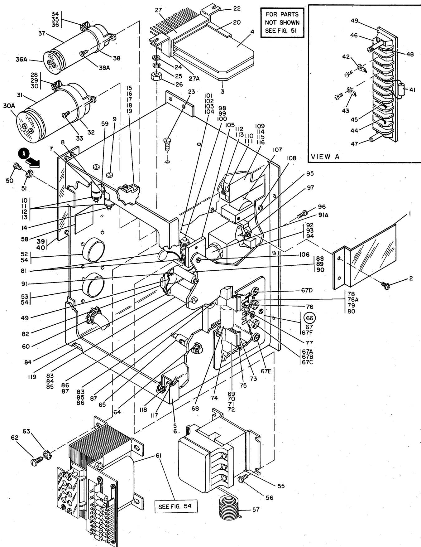
FIGURE 53. POWER SENSE AND BATTERY CHARGER ASSEMBLY.
