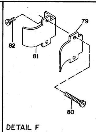
FIGURE 12. CPU FINAL ASSEMBLY-FRAME 02. (SHEET 1 OF 2, INDEX NOS. 1-97)
