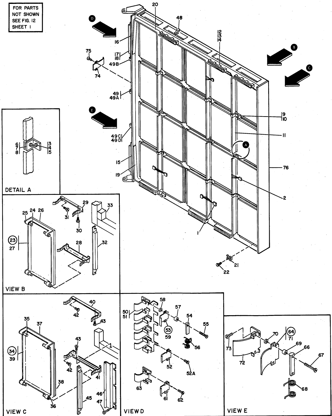
FIGURE 15. 8 GATE ASSEMBLY
