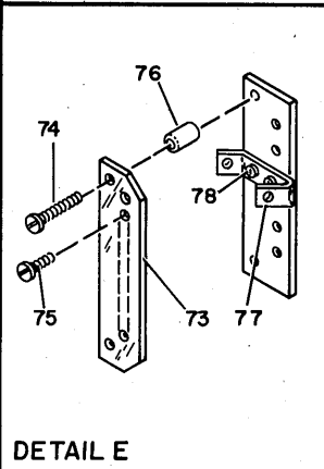
FIGURE 12. CPU FINAL ASSEMBLY-FRAME 02. (SHEET 1 OF 2, INDEX NOS. 1-97)
